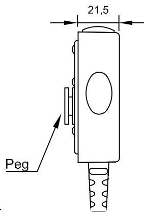
Microphone bracket
