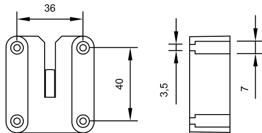
Microphone bracket
